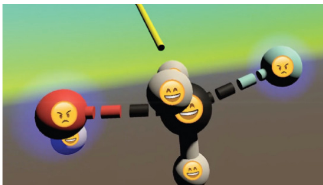
Figure 8: The emojis are used in IntraChem [SWF*21] to label happy/angry atoms based on a bond saturation. The image was adapted. Permission for re-use obtained.
