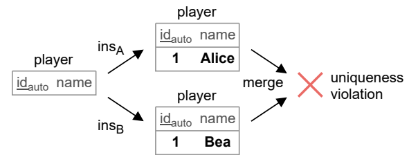
Figure 1. Uniqueness violation
