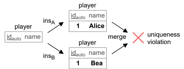
Figure 1. Uniqueness violation
