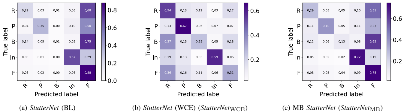
Fig. 5: Accuracy confusion matrices showing the confusion of fluent speech with repetitions and blocks. F: Fluent, R: Repetition, B: Block, P: Prolongation, In: Interjection, BL: Baseline, WCE: Weighted cross-entropy, MB: Multi-branch.
