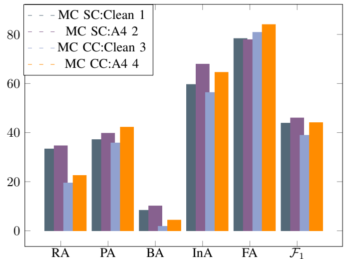
Fig. 6: Impact of data augmentation (A4) in cross corpora FluencyBank dataset with MC StutterNet (R: Repetition, P: Prolongation, B: Block, In: Interjection, F: Fluent, XA: X: Disfluency Class and A: Accuracy, MC: Multi contextual StutterNet , SC: Same corpora, CC: Cross corpora, A4: Augmentation). The bar plot clearly shows that the model MC StutterNet trained on clean SEP-28k dataset fails to generalize on FluencyBank cross corpora data. Applying data augmentation improves the stuttering detection in cross domain corpora as shown orange bars (4 th column in each disfluency).
