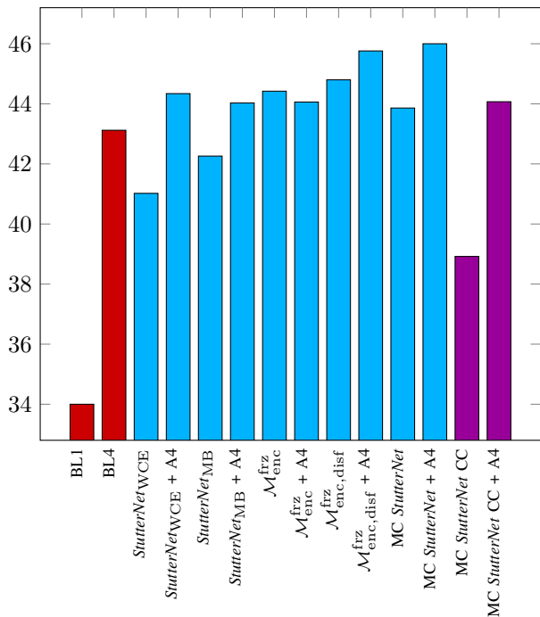
Fig. 7: Macro \mathcal{F}_1 score summary of proposed and baseline models (BL1 and BL4). The red, light blue and purple bars indicate the baseline, same-corpora setting, and cross-corpora settings. (CC: Cross Corpora with training on SEP-28k and evaluated on FluencyBank dataset, A4: All four data augmentation. The second last bar shows cross-corpora performance on FluencyBank when trained using a clean SEP-28k dataset and the last bar shows the same with data augmentation).
