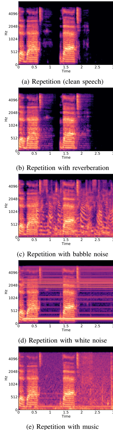
Fig. 2: Repetition stuttering with utterance "said that, that" and the effect of various data augmentations (From 0 to 0.25 seconds, the speaker is saying "said", then followed by two repetitions "that" from 0.25 to 0.6 and 1.4 to 1.75).
