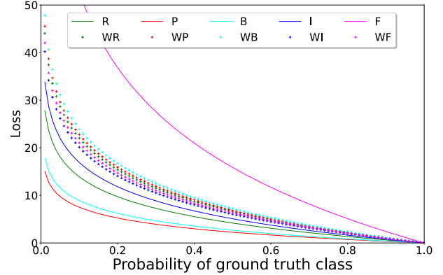
Fig. 4: Class-wise loss values for different probabilities of ground truth classes. Here block, fluent, repetition, prolongation, and interjection classes are correspondingly denoted by B, F, R, P, and I. The standard cross entropy (CE) is shown by solid curves and its weighted version is shown by dashed ones (WX represents the weighted loss of class X).
