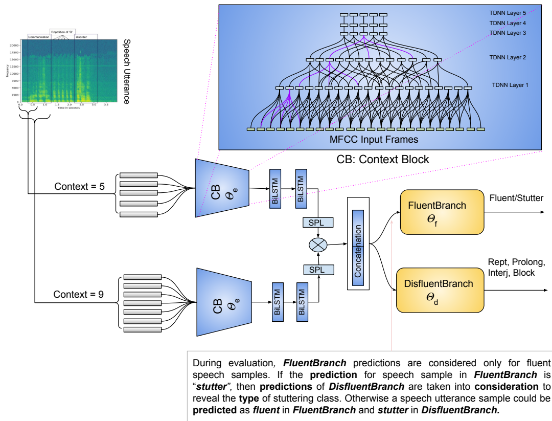
Fig. 3: A schematic diagram of Multi-contextual StutterNet , which is a multi-class classifier that exploits different variable contexts of (5, 9) in SD. The FluentBranch and DisfluentBranch are composed of 3 fully connected layers followed by a softmax layer for prediction of different stuttering classes, CB: Context Block, SPL: Statistical Pooling Layer. The context C (5, 9) here does not mean the TDNN layers, but rather it means the kernel-size which is number of frames taken into account when processing speech frames (C=5 means a context of 5 frames are taken at a time and C=9 means a context of 9 frames are taken at a time). These two contexts are jointly exploited in MC StutterNet as shown in the left hand side of the figure.
