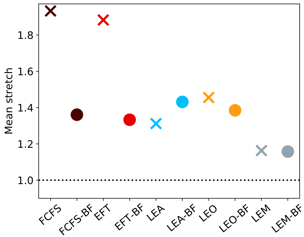
Figure 15: Average stretch of all jobs evaluated on January 28 with (circles) and without (crosses) backfilling.
