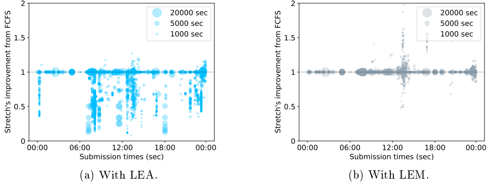
Figure 5: Stretch times of each job compared to FCFS on the workload of July 16.
