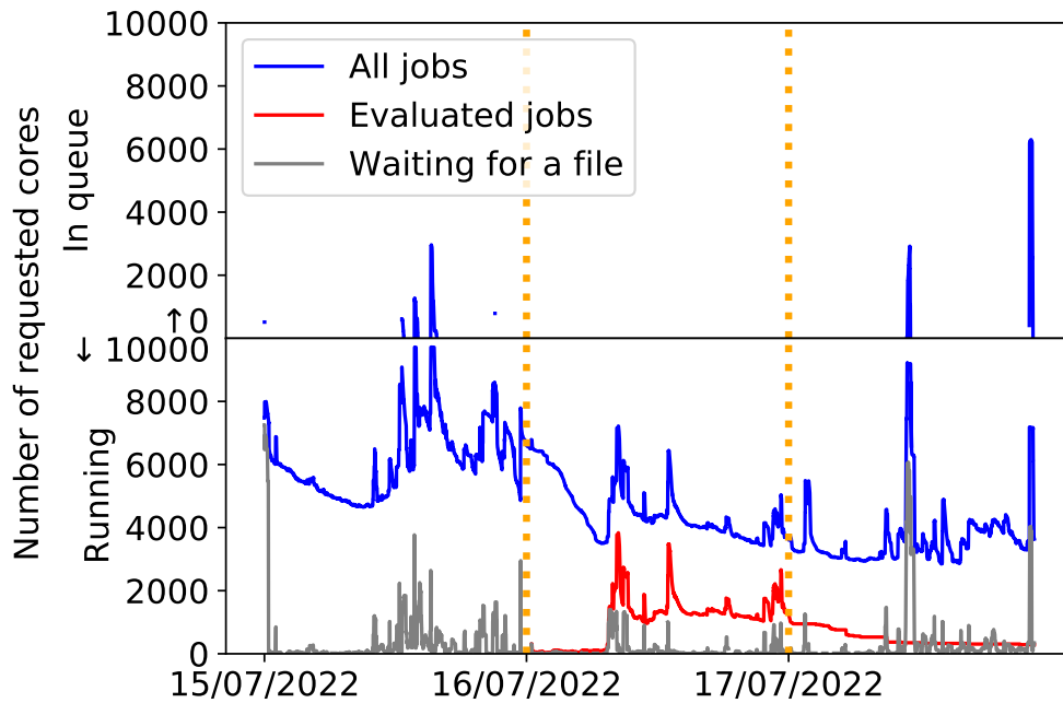
Figure 3: Visualization of the utilization rate of the cluster on the workload of July 16 with FCFS.
