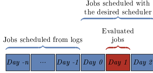
Figure 1: Methodology followed to schedule and evaluate jobs from a specific day while avoiding edge effects.
