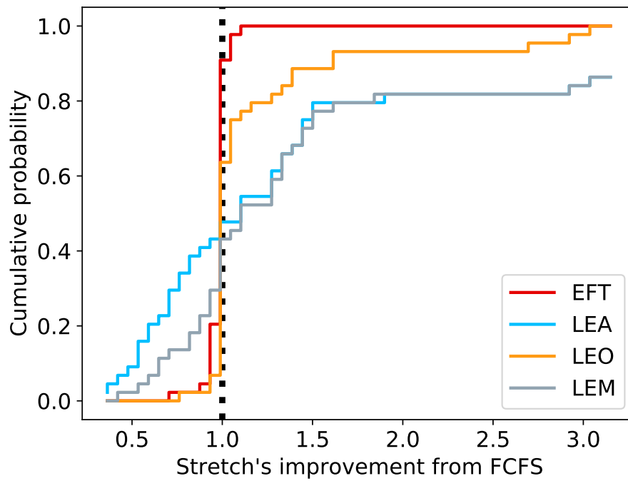
Figure 14: Empirical distribution function of the mean stretch's improvement from FCFS on all evaluated workloads.
