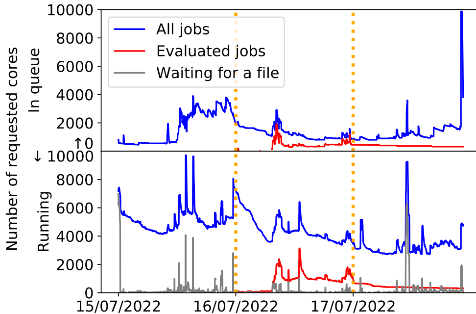
Figure 4: Visualization of the utilization rate of the cluster on the workload of July 16 with LEA.
