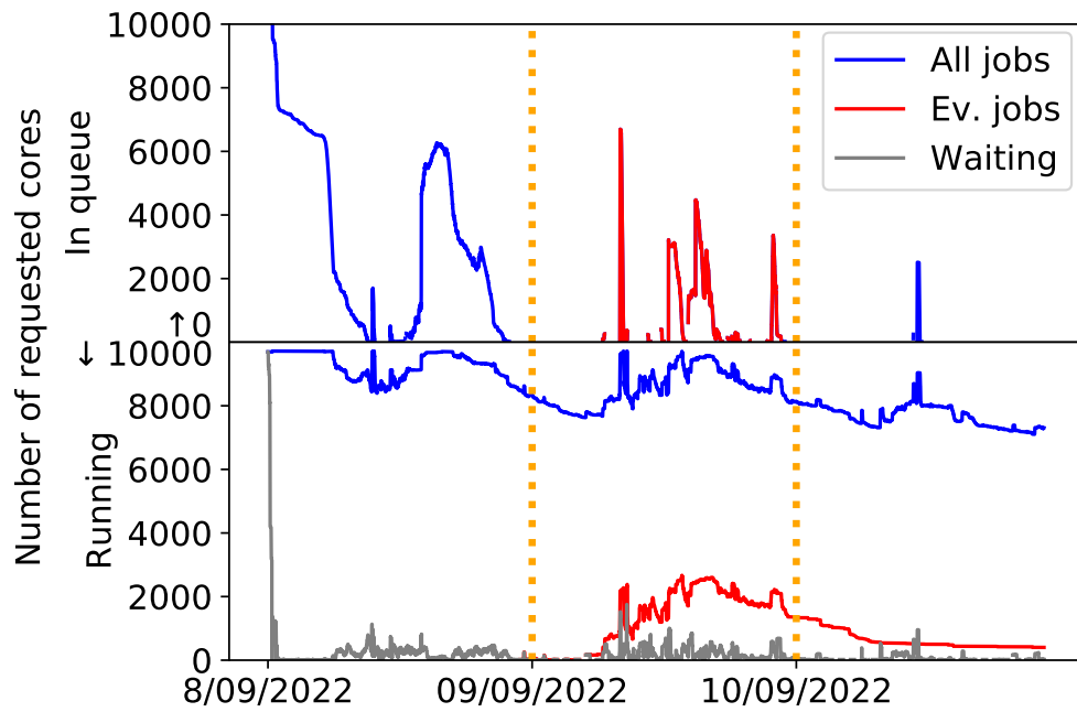
Figure 7: Visualization of the utilization rate of the cluster on the workload of September 9 with FCFS.
