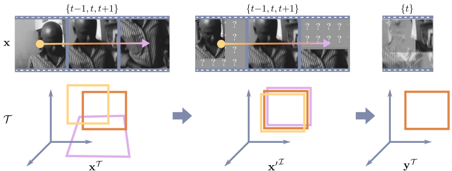
Fig. 8. Illustration of our implementation of WorldFeatures. We start with a world feature map \mathbf{x}^\mathcal{T} and in order to calculate the output of a convolution applied to the feature map at time t , that is \mathbf{y}^\mathcal{T}(t, h, w) , we first transform the needed features into the coordinate system at time t , and then apply the convolution as normal. Black, gray and white, are used to denote t-1 , t , and t+1 , respectively.
