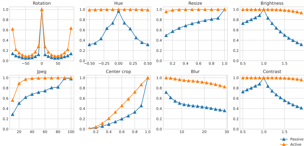
Figure 8: Average R@1 comparison between active and passive indexing with IVF-PQ.
