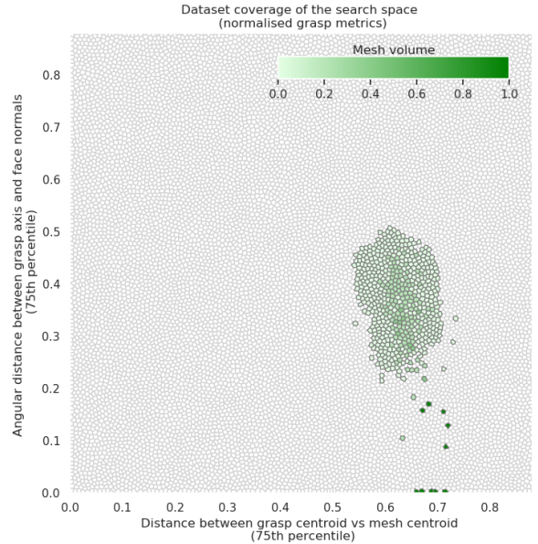
(a) Coverage of the projection space by our (AGOD) dataset
