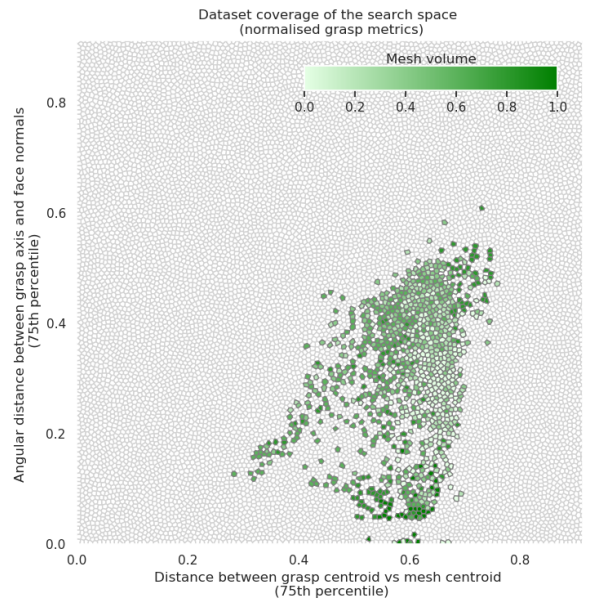
(b) Coverage of the projection space by EGAD dataset [22]
