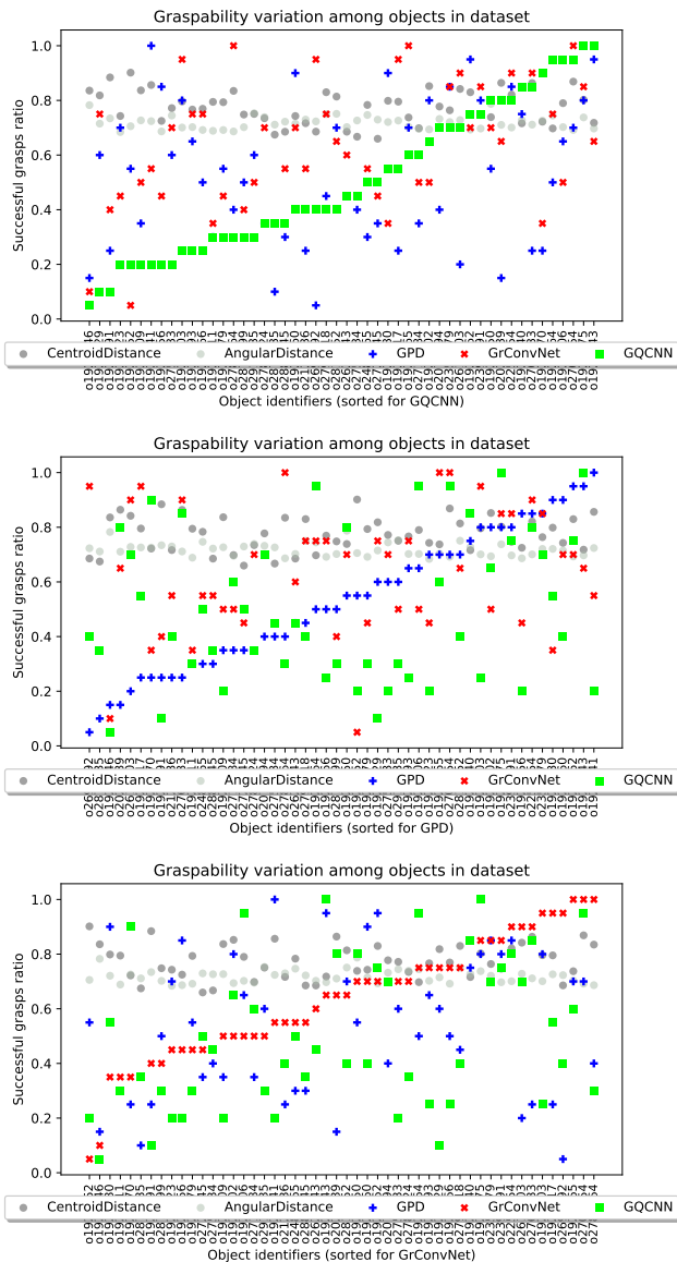
Fig. 7: Grasability variation among generated objects. Each plot presents the same objects, but sorted according to graspability scores obtained using a specific algorithm (GPD/CQCNN/GrConvNet). Generated objects cover almost the full graspability range of these algorithms. The gray dots correspond to predicted graspability scores.
