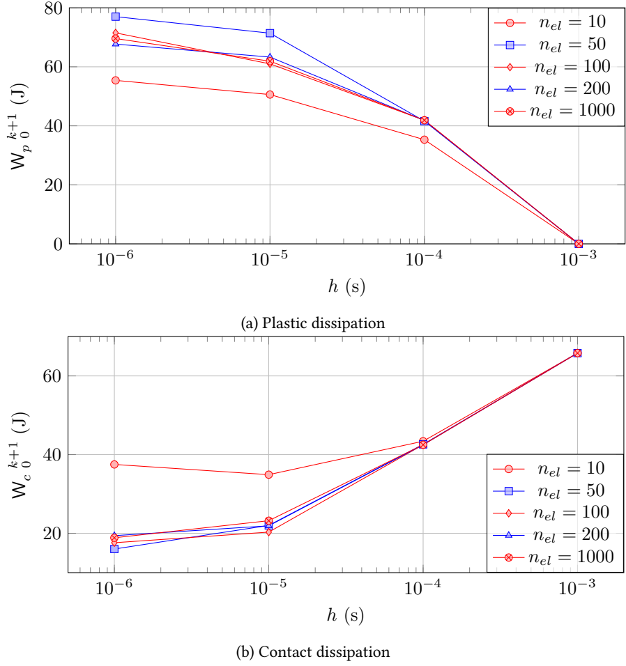
Figure 21: Example 2: Convergence of the energy dissipated by plastic flow (a) and contact (b) after the end of the first phase of intermittent interactions between the sphere and the cantilever beam (end of the light blue area on Figure 20). The dissipated energies are plotted as a function of the time step h for different numbers of elements n_{el} .
