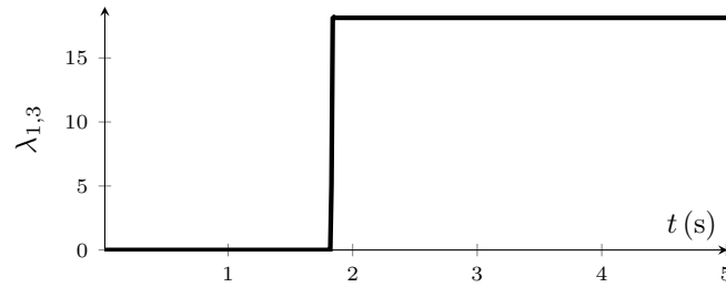
Figure 8: Example 1, case 1: time evolution of the plastic multipliers \lambda_{1,3} at Gauss point 1 of the cantilever beam subjected to axial and transversal displacements simultaneously in the case of perfect plasticity.
