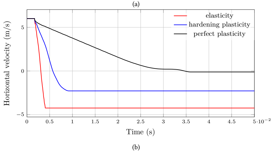
Figure 24: Example 3: Projectile and structure impacted point horizontal positions (a) and projectile velocity (b) as a function of time for different material constitutive and evolution laws (elasticity, perfect plasticity and hardening plasticity).
