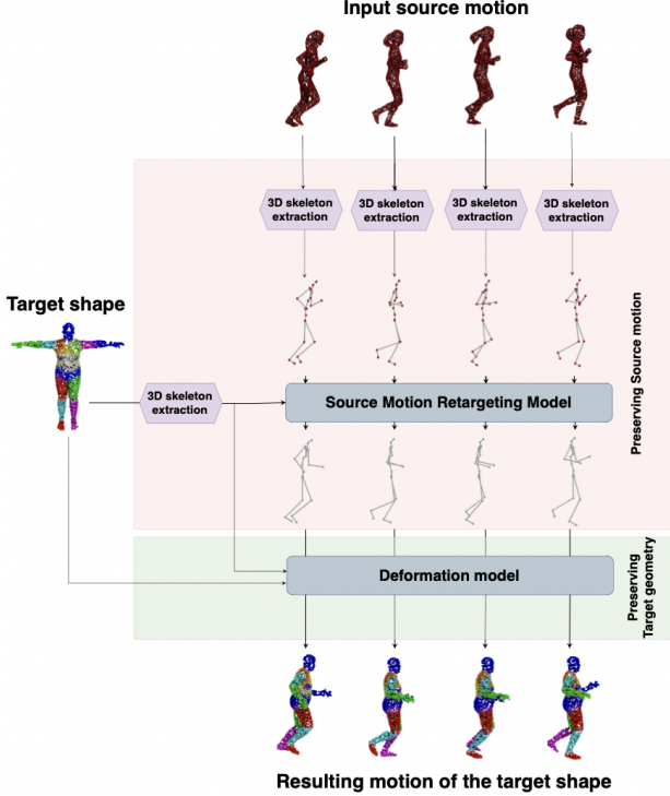
Figure 2. Our method takes a source sequence of unstructured point clouds and a target point cloud as input, and outputs the target character performing the input motion. The method first retargets the source motion to the target character at the skeletal level (red part), and then adds the target’s surface details to the resulting motion using a deformation model (green part).
