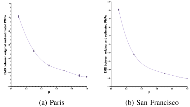
Figure 10: (a) and (b) illustrate that EMD between the true and the estimated distributions of the locations in Paris and San Francisco, respectively, after the empirical convergence of PRIVIC for the different values of the loss parameters \beta .
