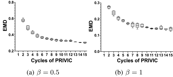
Figure 8: (a) and (b) show the EMD between the true PMF of the Paris locations and its estimation by PRIVIC in each of its cycle for \beta = 0.5 and \beta = 1 , respectively.
