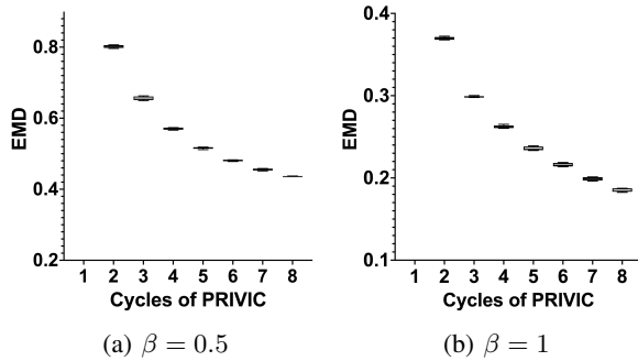
Figure 9: (a) and (b) show the EMD between the true PMF of the San Francisco locations and its estimation by PRIVIC in each of its cycles for \beta = 0.5 and \beta = 1 , respectively.
