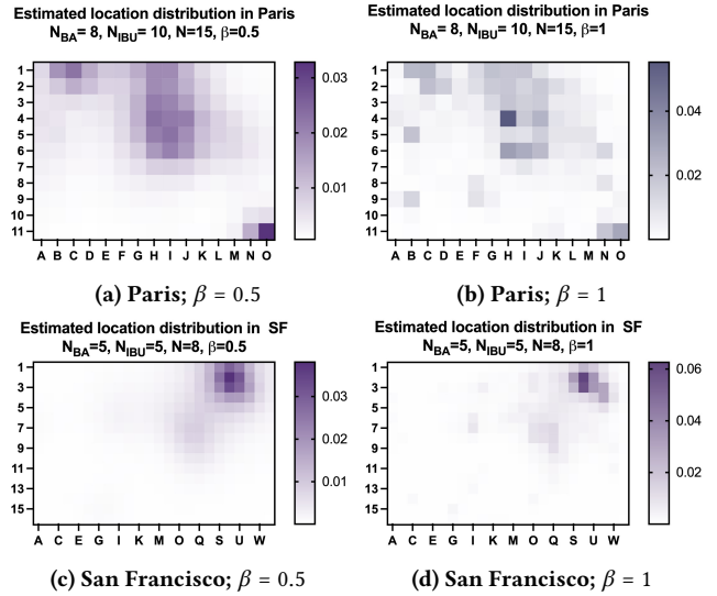
Figure 7: Visualization of the estimated true distribution of the locations in Paris ((a) and (b)) and San Francisco ((c) and (d)) by PRIVIC after its convergence; the first column is for \beta = 0.5 and the second column is for \beta = 1 .
