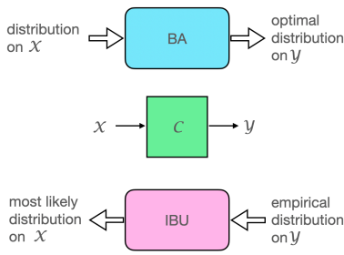
Figure 4: Illustration of the duality between BA and IBU.
