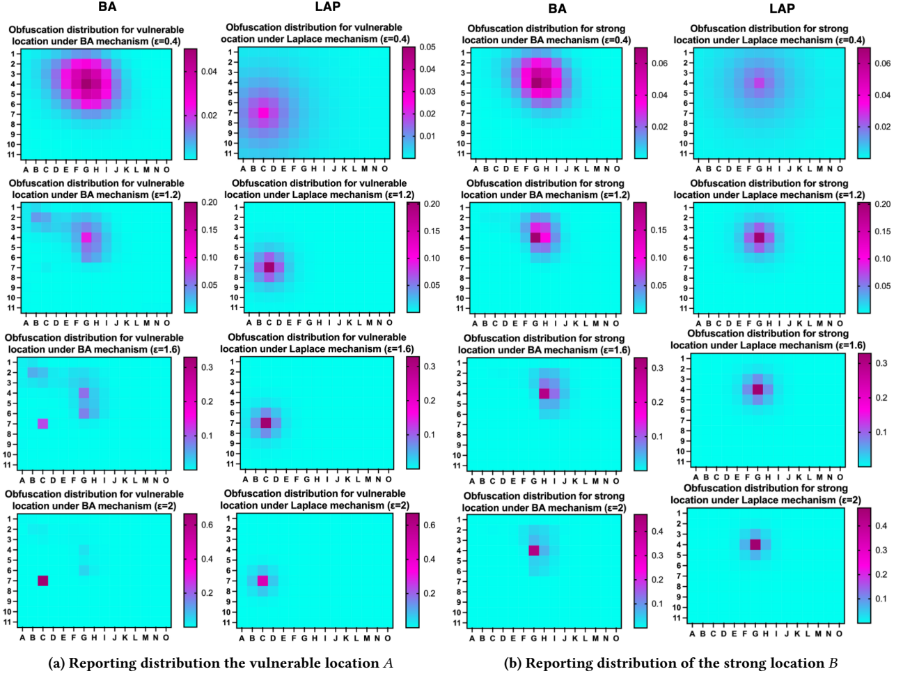
Figure 2: Distribution of privatizing the vulnerable and the strong locations for different levels of privacy. Top down, the rows illustrates the results for \epsilon = 0.4, 1.2, 1.6, 2 , respectively.
