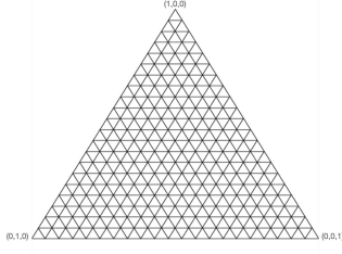
Figure 5: A visualization of a discretized simplex on \mathcal{X} of size 3 showing that the continuous simplex (the entire area inside the triangle) has been made finite with the mesh.
