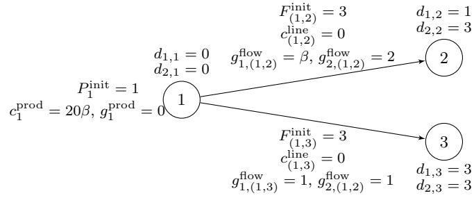
Figure 7: An instance with 3 nodes, 2 arcs, 2 scenarios ( p_1 = 0.9 and p_2 = 0.1 ), 1 time unit, and such that V = 10\beta , \epsilon = 0.1 , \alpha = 1.5 .
