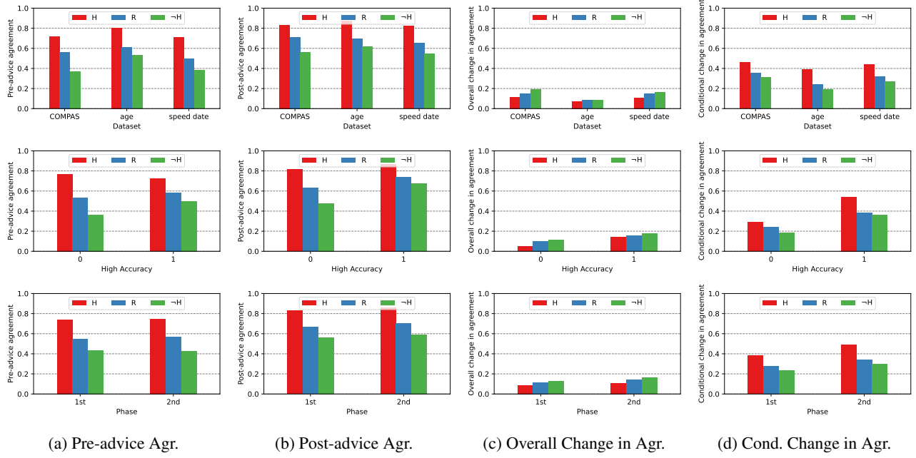
Figure 12: Influence of machine advice on respondents' agreement with the advice, for decision aids with human-like (H), anti human-like ( \neg H ), and randomly distributed (R) errors. The results are separated by dataset [top], accuracy [middle], and phase [bottom]. Across all three control variables, pre and post-advice agreement, and the conditional change in agreement are higher for human-like decision aids than for anti human-like decision aids. On the other hand, for the overall agreement, the opposite pattern holds.
