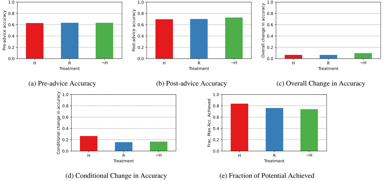
Figure 5: Influence of machine advice on respondents' accuracy , for decision aids with human-like (H), anti human-like ( \neg H ), and randomly distributed (R) errors. Pre and post-advice accuracy, and the conditional change in accuracy are higher for human-like decision aids than for anti human-like decision aids. Human-like decision aids were also closer to reaching their full potential in terms of improving the respondents' accuracy. However, for the overall change in accuracy, the opposite holds.
