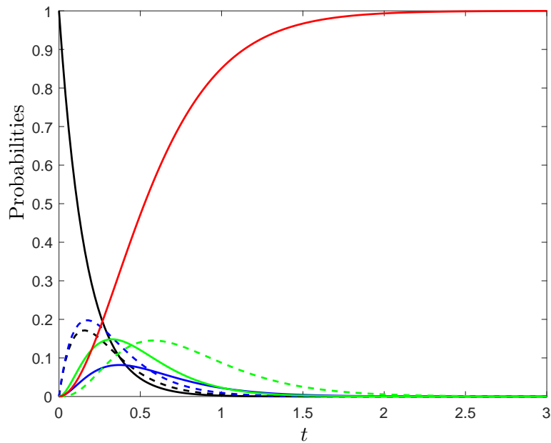
Figure 20: Transient state probabilities of the states of the CTMC as a function of time t , t \in [0, 3] , for p = 2 , r = 6 and C = 3 , with \rho = 0.8 , \lambda = 3 and so \mu = 0.625 .
