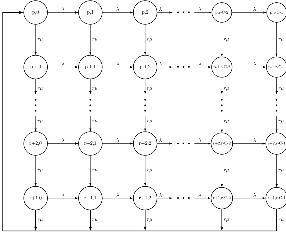
Figure 23: Irreducible CTMC modeling the execution of an infinity of independent realizations of the August's waiting time distribution.
