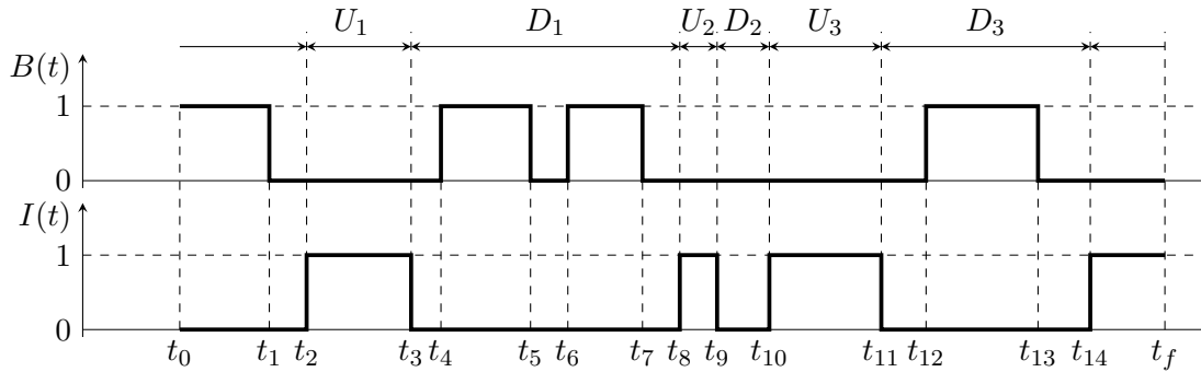
Figure 11: Partial trajectories of B(t) and of I(t) over a time interval between t_0 and t_f .
