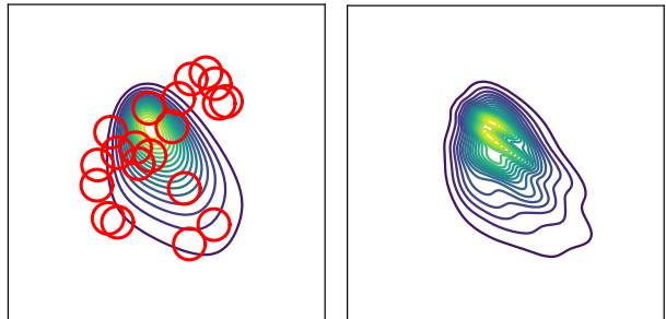
Figure 1: Left: randomly initialized mixture of 20 Gaussians (the initial covariances are depicted as red circles) and contour plot of a logistic target \pi . Right: contour lines of a mixture of Gaussians approximation \hat{\pi} obtained from the gradient flow in Section 5.
