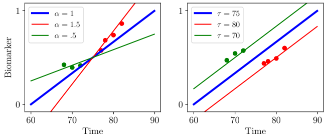
Fig. 1. Illustration of the mixed-effect model with time-warp. Blue curve is the average trajectory (parameterised by t_0 , p_0 and v_0 ) and red and green curves illustrate the effect of progression pace ( \alpha = e^\xi ) and onset age ( \tau ) to match individual measurements (isolated dots) to a continuous trajectory.
