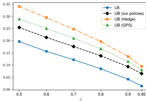
Figure 9 Upper bounds on the optimal average discounted regret achieved by the different policies plotted as a function of the discount factor \beta . Also plotted is the theoretical lower bound on regret.
