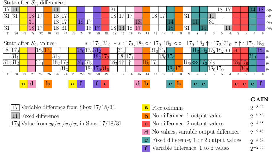
Fig. 3: Reducing the required keybit guesses in the first round.
