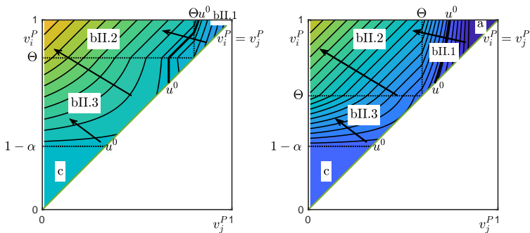
Figure: Level curves for utility: \varepsilon = 0.7 (left), \varepsilon = 0.4 (right).
