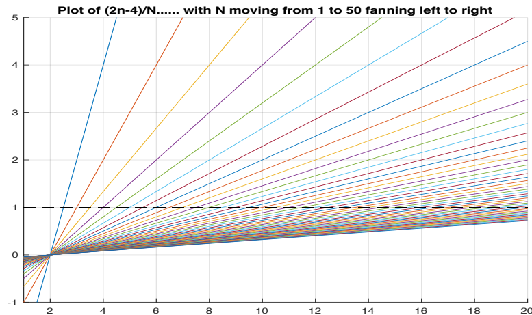
Figure 2: Existence of moments for the VEnKF . Each line corresponds to some number N with N moving from 1 to 50 fanning left to right. The ‘x-axis’ corresponds to moment orders n and a moment n exists whenever the line (2n - 4)/N is strictly less than one.
