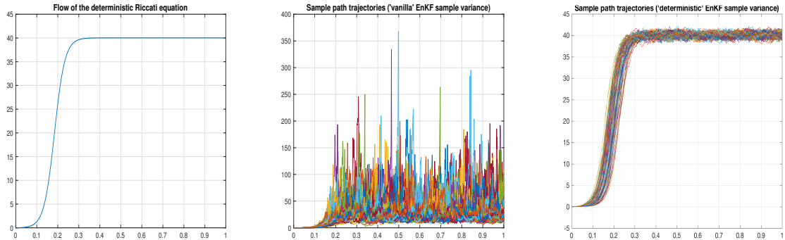
Figure 4: Flow of the deterministic Riccati equation, and 100 sample paths of the VEnKF sample variance of case (F1), and 100 sample paths of the DEnKF sample variance of case (F2).
