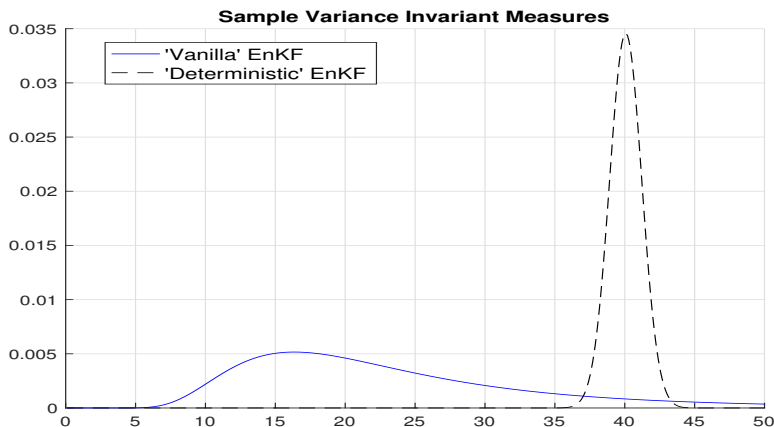
Figure 3: The invariant measure of the sample variance of the ‘vanilla’ EnKF in case (F1), versus that of the ‘deterministic’ EnKF in case (F2).
