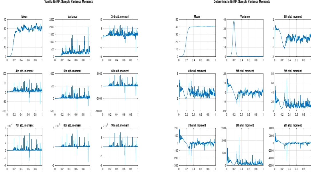
Figure 5: Flow of the sample variance moments for the VEnKF and the DEnKF.
