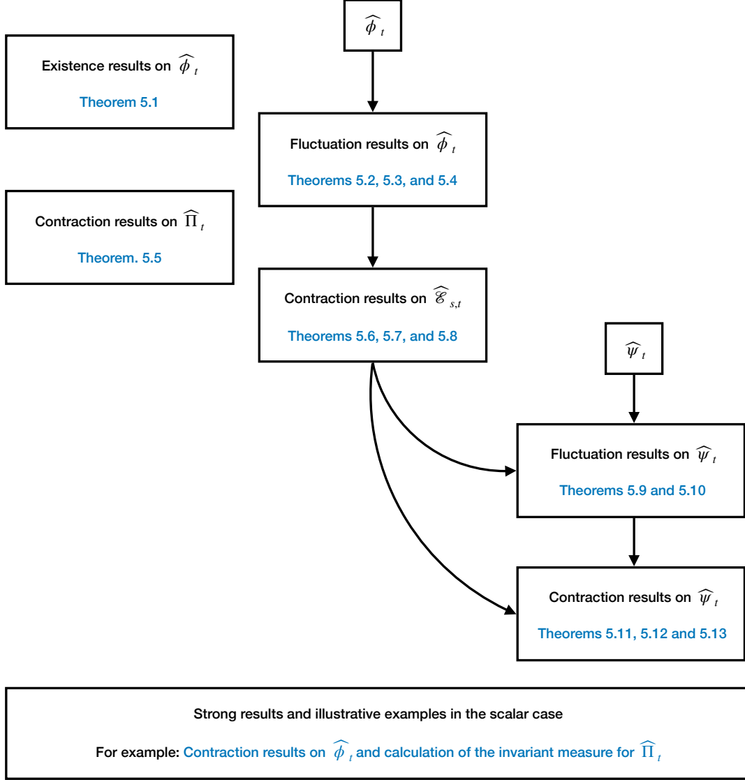
Figure 1: Flowchart of the general result and topics in this article. Although detailed proof in most cases is not given, the arrows and top-down direction in the flowchart depict both the presentation of the results in this article, and the dependency in terms of the proof and derivation of the results
