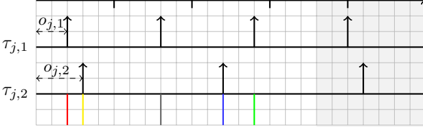
Figure 4: A transaction with two tasks. Their offsets are 2 and 3, their periods are 6 and 9, respectively. The LCM of task periods is 18, during which there will be 5 activations. This transaction, therefore, represents 5 alignments. Each vertical colored line indicates an alignment.
