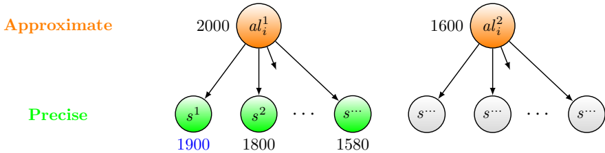
Figure 6: Scenario domination according to the two-level combined analysis for a system of four transactions. Each approximate scenario (orange node) dominates 8000 precise scenarios (green nodes). Unprinted nodes and the nodes in grey represent the scenarios which do not need to be analyzed.
