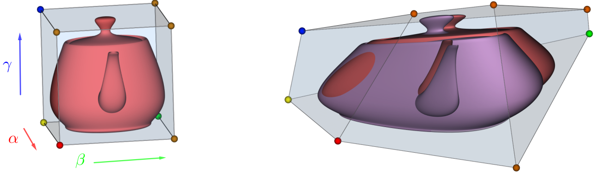
FIGURE 2: Left: we choose freely positive values for w_{000}, w_{100}, w_{010}, w_{001} and compute constants \alpha, \beta, \gamma that allow us to derive the remaining w_{ijk} 's while preserving the weight ratio in each direction of the space. Right: A hexahedral FFD with all the w_{ijk} 's equal to 1 (red), and w_{ijk} 's computed using Theorem 2 (purple). In the second case, the FFD is birational although the deformation has not changed significantly.
