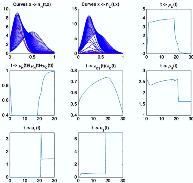
Fig. 1. Evolution with time t of the x resistance phenotype distribution curves n_H(t, x) and n_C(t, x) and solution (u_1, u_2) of the OCP problem for T = 30 . In the lower two panels, one can see that the cytotoxic drug u_1 level is maintained positive, but as low as possible, close to zero, for a long time, before delivering its maximal tolerated dose on a short time interval, so as to keep the cell population as sensitive as possible until time T_1 (here T_1 \approx 20 ) - which is the drug holiday strategy used in the clinic of cancers [54] -, then delivered at a medium dose. The cytostatic drug u_2 level is maintained at a low level, but not close to zero, until some time before and close to T_1 , and then delivered at its maximum tolerated dose. One can see on the two rightmost panels that the cancer cell population \rho_C goes to extinction while the healthy cell population \rho_H is preserved over a prescribed level. The central panel shows an evaluation of the ratio of drug-sensitive cancer cells \int_0^1 (1-x)n_C(t, x)dx over total cancer cells. Performed in modelling language AMPL with expert simulation routines IpOpt. Adapted from [47] with permission.
