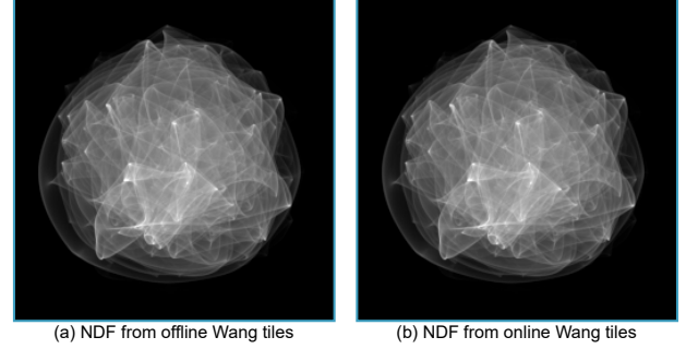
Fig. 14. We visualize the NDF of a normal map generated by Wang tiles offline (generate the synthesized normal map explicitly) and online (using the color hash table to generate the synthesized normal map implicitly).
