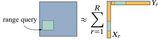
Fig. 6. Angular range query (green box) is performed on the compressed tensors. The average value in a rectangle can be decomposed as the product of the average values along its axis green segment on the right image).
