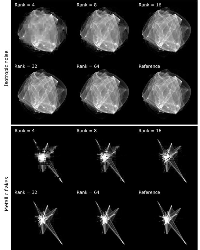
Fig. 19. Reconstructed NDF images from tensor decomposition with varying ranks. We set the rank as 16 for isotropic noise and 32 for metallic flakes, balancing both the quality and the storage. Normal map: isotropic noise and metallic flakes.
