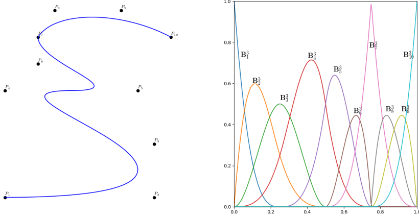
FIGURE 2. (left) A cubic B-Spline curve and its control points using the knot vector \Xi = \{0000 \frac{1}{4} \frac{1}{2} \frac{3}{4} \frac{3}{4} \frac{3}{4} \frac{3}{4} 1111\} , (right) the corresponding B-Splines.
