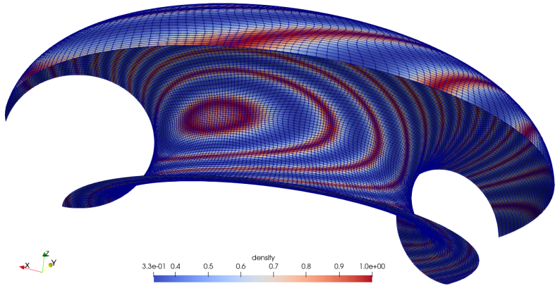
FIGURE 18. Adaptive meshes and the monitor function.
