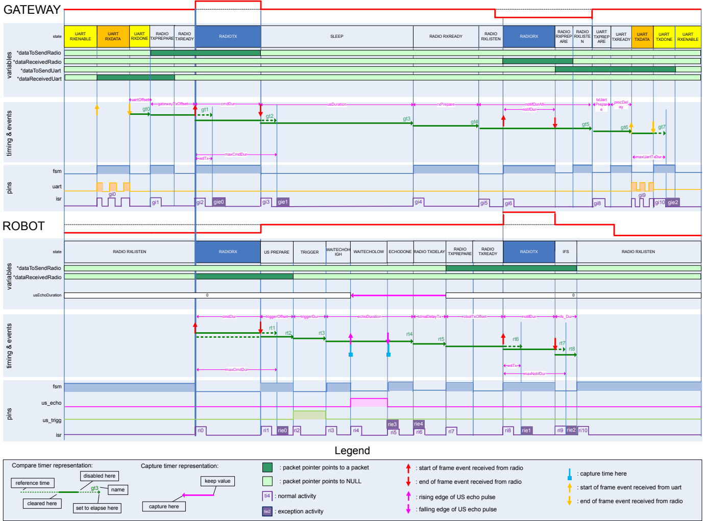
Fig. 5. Chronogram of the RRDV state machine representing the activity of a gateway and mobile robot. The figure shows their radio activity (red line), events and timers, value of the global variables and the state of the debug pins.
