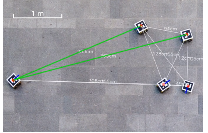
Fig. 1. In our experimental evaluation, five robots drive around randomly. RRDV detects when two robots are facing one another. We call this an “encounter”; it is depicted as a green line.
