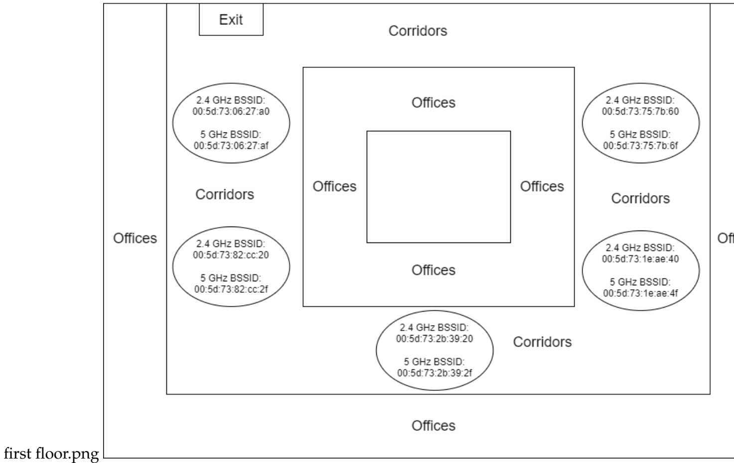
Figure 7.2: Lagrange building, first floor
