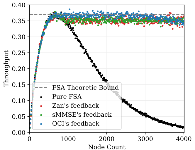
(a) Throughput with 75% effective detection
