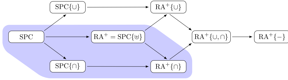
Fig. 1. Summary of the results. An edge indicates a more expressive fragment. Adding duplicate elimination makes every fragment more expressive, and incomparable with RA^+ \{-\} . Extending RA^+ \{-\} with duplicate elimination results in a fragment that has the expressive power of full RA. The shaded area includes the fragments for which computing the minimum occurrences of certain answers is tractable, while this is intractable whenever duplicate elimination is added. Computing the maximum number of occurrences is intractable for all fragments.
