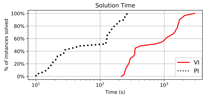
Fig. 3. Solution time performance profile.
