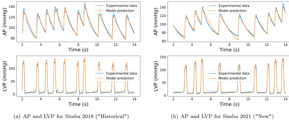
FIGURE 6. Experimental data compared with the model prediction for Simba.
