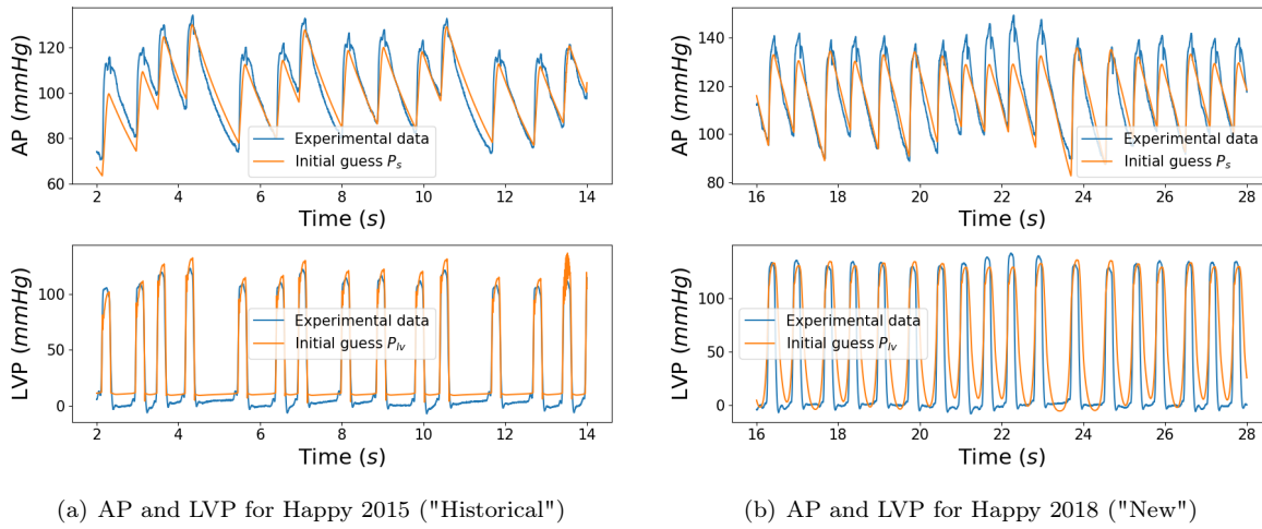
FIGURE 7. Experimental data compared with the model prediction for Happy.
