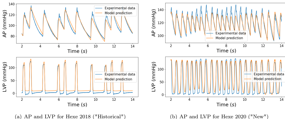
FIGURE 8. Experimental data compared with the model prediction for Hexe.
