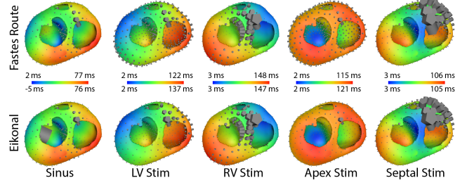
Figure 2. Predicted mean and standard deviation of the LATs. Max standard deviation is 84 ms (septal stimulation) for the fastest route model and 114 ms (sinus) for the Eikonal model.
