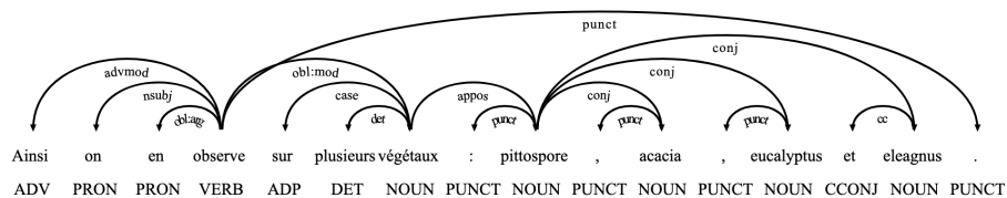
Fig. 3. Stanza's Dependency Analysis
