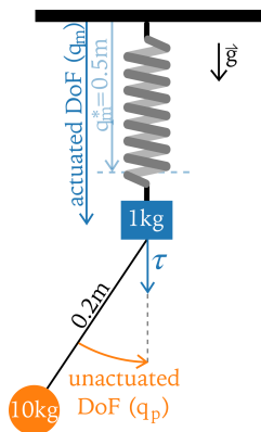
Fig. 6. Spring-mass-pendulum model of Ex. C.
