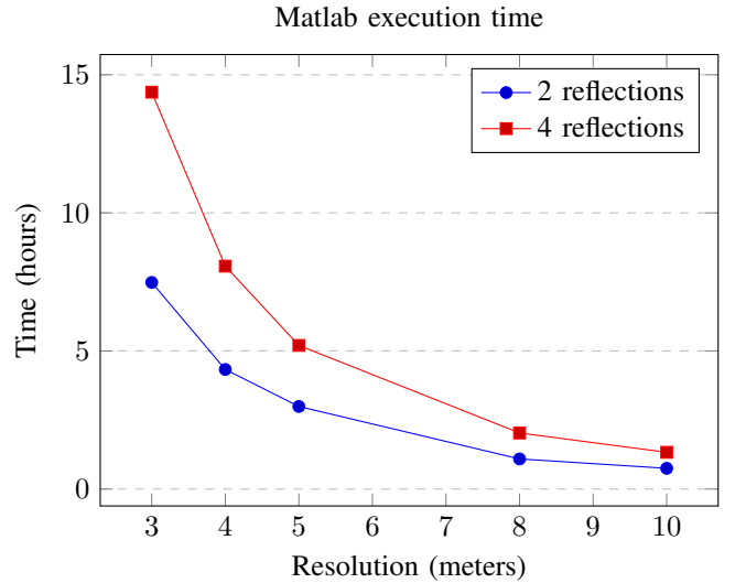
Fig. 6. Matlab execution time
