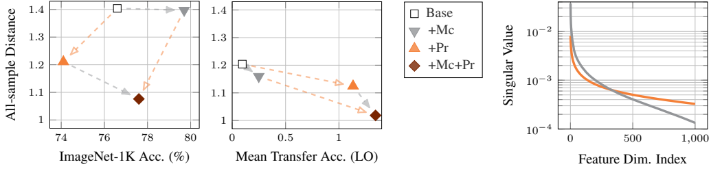
Figure 13: (left) All-sample \ell_2 distance vs. performance on IN1K and transfer datasets. These two sub-plots extend the intra-class distance plots shown in Fig. 5 (left) of the main paper. Gray and Orange arrows denote changes due to adding multi-crop and projectors, respectively. (right) Singular values across dimensions, averaged over the transfer datasets. We show the first 1000 dimensions (of 2048) for clarity.
