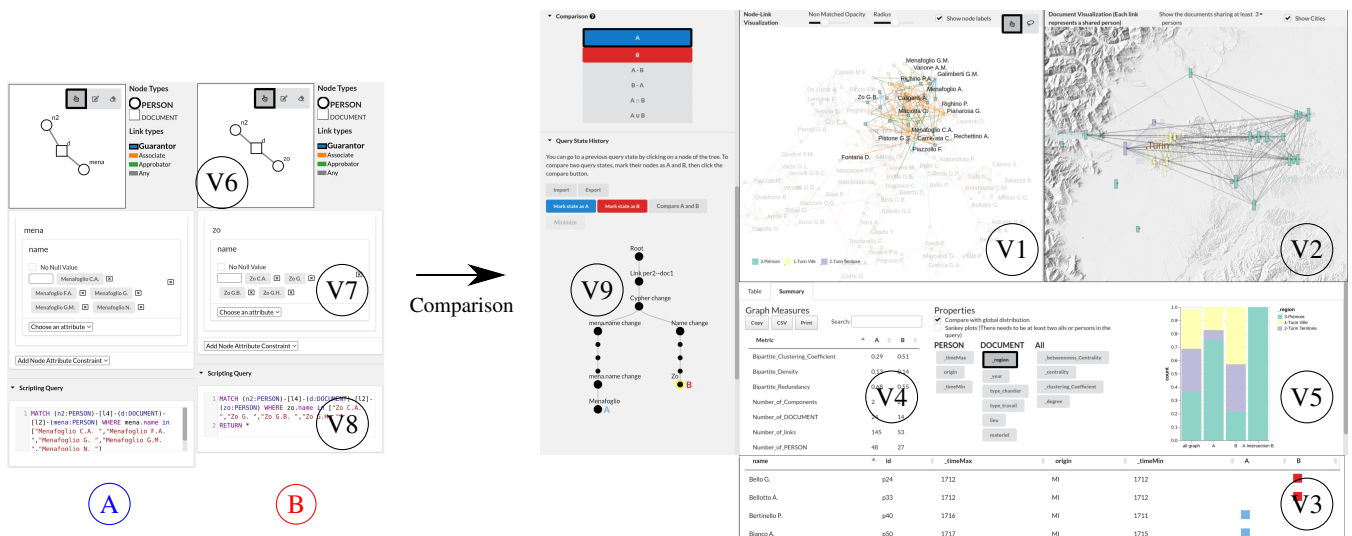
Figure 1: The ComBiNet system used to compare two subgroups of a social network of contracts from [CR18], extracted with dynamic visual queries. (A) and (B) show the two visual queries created by the user in the query panel using an interactive node-link diagram editor (V6), dynamic query widgets (V7), and the equivalent Cypher script (V8). The right part shows ComBiNet’s global interface in comparison mode: (V1) Network visualization panel, (V2) Map of the geolocalized nodes, (V3) Table of persons, (V4) Graph measures comparison, (V5) Attribute distribution plots, and (V9) Provenance tree. The two visual queries on the left, select the “Menafoglio” family on the left, and the “Zo” family on the right, along with their construction contracts and close collaborators.
