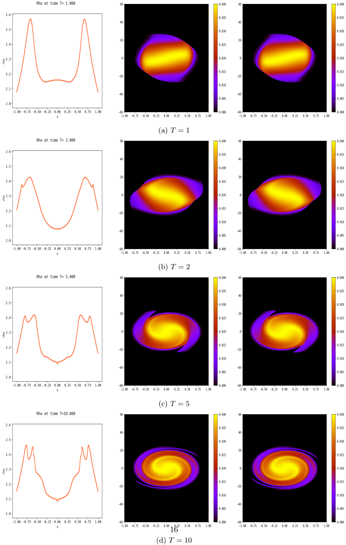
Figure 10: Density \rho (left) and electron distribution function (middle and right) for time T \in \{1, 2, 5, 10\} ; The semi-Lagrangian code is used with parameters of Run2 (left, middle) and of Run3 (right).
