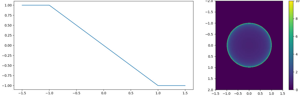
Figure 1: Malkov solutions (3.4) on [-1.5, 1.5] \times [-2, 2] . Left: electric field E . Right: density f .
