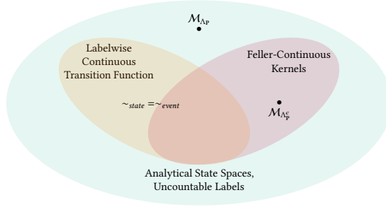
Fig. 3. LMP-equivalences for Analytical States Spaces and Uncountable Labels
