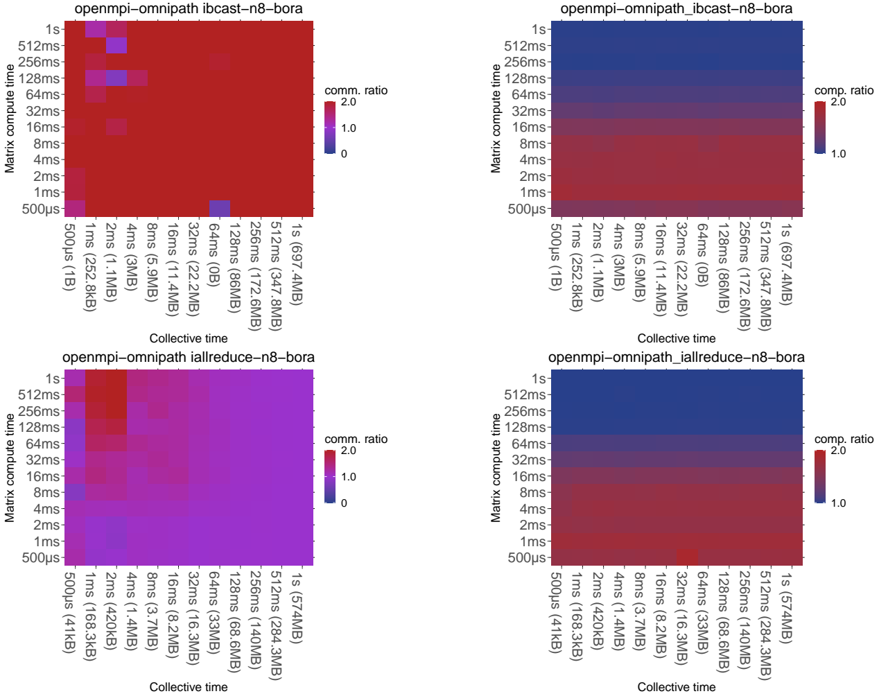
FIGURE 20 OpenMPI concurrency ratios r_{comm} (left) and r_{comp\_slowdown} (right) on Omni-Path on 8 nodes
