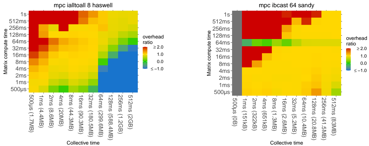
FIGURE 17 MPC overlap results on InfiniBand for MPI_Ialltoall and MPI_Ibcast on 8 nodes (left) and 64 nodes (right)
