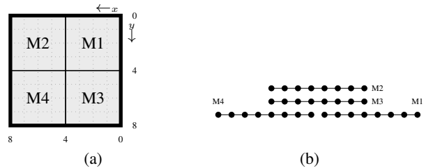
Fig. 3: Tiling (a) and dot diagram (b) of a 8 \times 8 -multiplier, composed of four 4 \times 4 sub-multipliers M_1 \dots M_4 .
