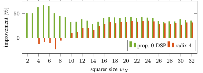
(b) LUT improvement compared to a radix-2 squarer
