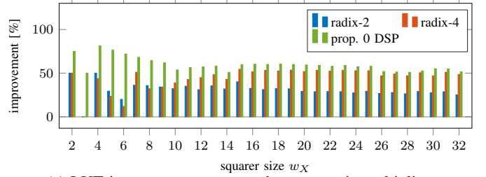
(a) LUT improvement compared to a generic multiplier
