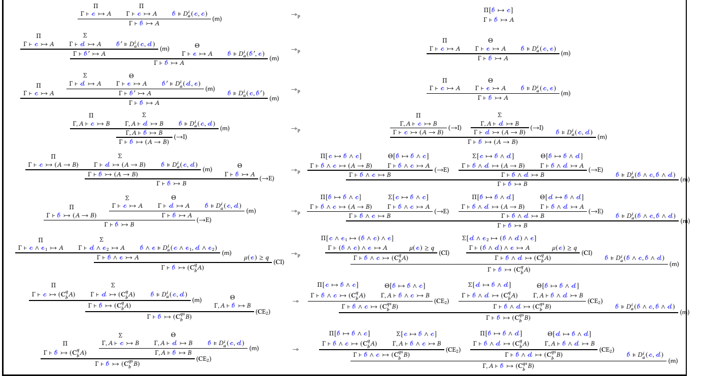
Figure 11. Permutative rules of \text{ND}_{\text{iCPL}_0} .
