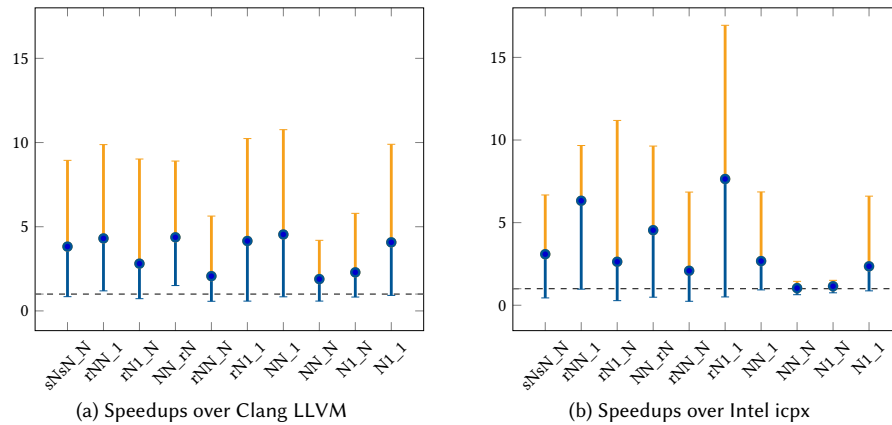
Fig. 13. Comparison of Autoveesk's automatic vectorization speedups against the Clang LLVM-based and Intel icpx compilers on 10 selected kernels. Each kernel was executed with different problem sizes. The minimum, average and maximum speedup over the compilers' auto-vectorization techniques are shown.
