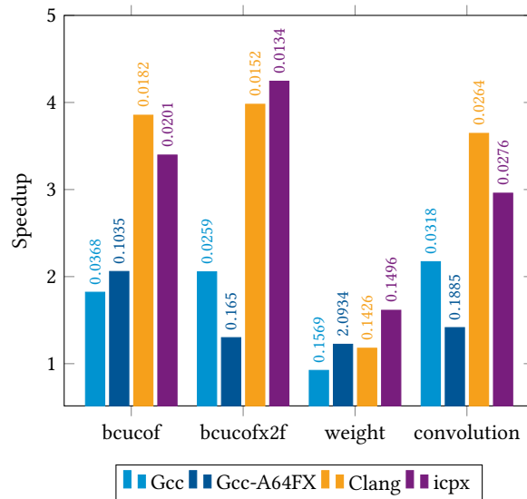
Fig. 14. Comparison of Autoveesk's automatic vectorization speedup against the GNU compiler (GCC) on x86 architecture and A64FX 64-bit ARM architecture, Clang LLVM-based compiler and the Intel (icpx) compiler for 4 different numerical kernels. We provide the execution times of the Autoveesk versions above each bar.
