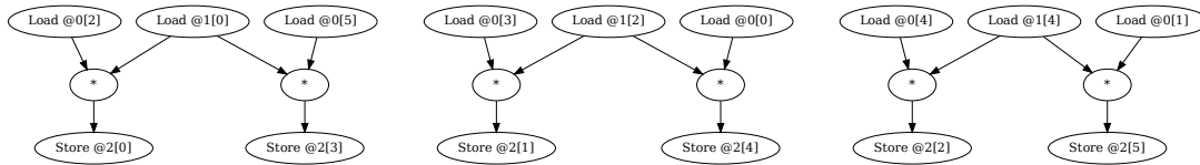
(a) Scalar graph for KA
