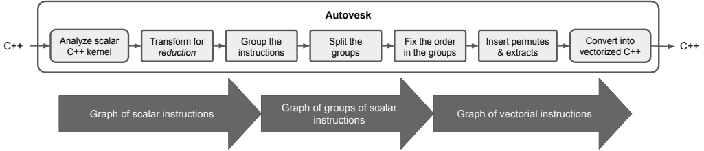
Fig. 1. Overview of the transformation flow in Autovesk. Starting from a C++ code, the tool successively uses a graph of scalar instructions, a graph of groups and a graph of vector instructions.
