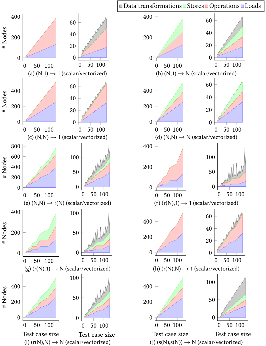
Fig. 12. Number and types of graph nodes for the different kernels and different problem sizes. The data transformation operations only exist for the vectorized kernels because they apply to vectors. The number of resulting binary instructions can differ but will be highly correlated to the numbers shown. A side-by-side comparison between the results of the scalar source code (left side) and the vectorized generated code (right side).
