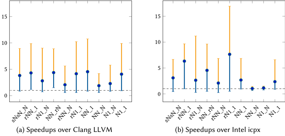
Fig. 13. Comparison of Autovesk’s automatic vectorization speedsups against the Clang LLVM-based and Intel icpx compilers on 10 selected kernels. Each kernel was executed with different problem sizes. The minimum, average, and maximum speedsups over the compilers’ auto-vectorization techniques are shown.
