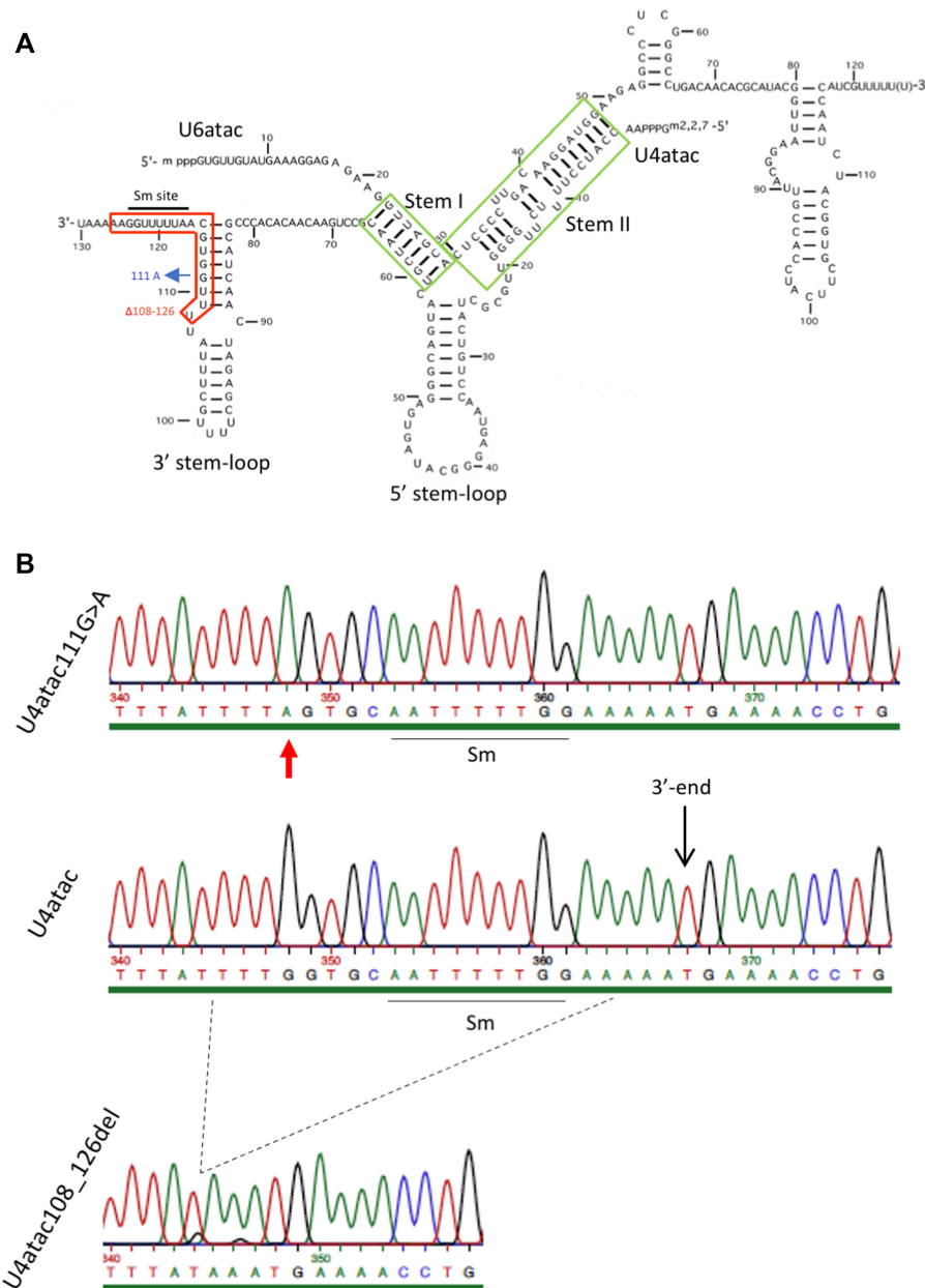
Figure 1. (A) Secondary structure of the human U4atac/U6atac snRNAs. The mutations found in the compound heterozygous g.108_126del:g.111G>A RNU4ATAC twin sisters are shown in red and blue. Adapted from Padgett and Shukla (91). (B) Sequencing chromatograms showing mutations in cloned DNA extracted from immortalized lymphoblastoid cells derived from compound heterozygous RNU4ATAC patients. The corresponding wild-type sequence from the control is shown in the middle. The Sm site essential for Sm core complex binding and snRNA stability is underlined. The 3' end of the wild-type U4atac is indicated. The position of the 111G>A mutation in the mutant is shown by a red arrow and the 108_126 deletion by dashed lines.
