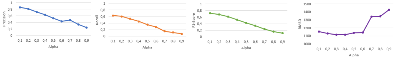
Figure 2: Metrics evolution according to different \alpha -cuts
