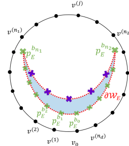
Figure 6: Non-convexity \partial\mathcal{W}_E : sudden jump from p_E^{b_{n_1}} to p_E^{b_{n_2}} .
